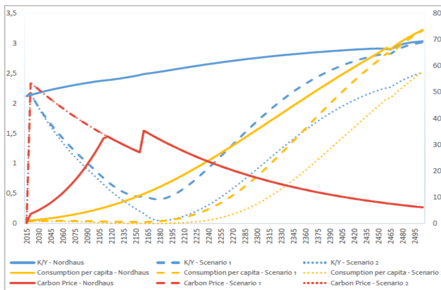
Figure 8. Simulated capital-to-output ratio (left axis, years), consumption per capita (right axis, thousand USD2005 per year), and carbon price (right axis, USD2005 per ton) in the DICE model for different specification of the damage function coefficient: Nordhaus ( a = 0.00236 ), Scenario 1 ( a = 0.16236 ) and Scenario 2 ( a = 0.18236 ).
