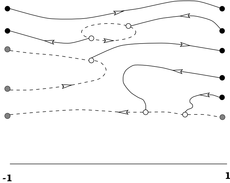
FIGURE 1. The parameterized moduli space W_\rho^* \cup W_\rho^r projecting vertically to [-1, 1] .
