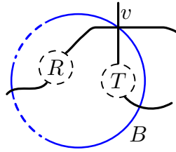
FIGURE 13. A cutting disk for D' .
