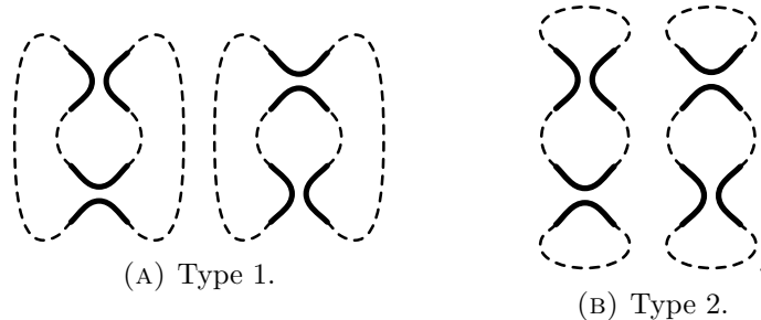
FIGURE 15. Non-alternating states on 2-crossing shadows of type 1 and 2.
