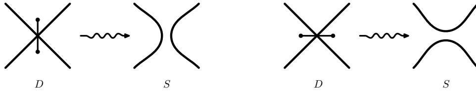
FIGURE 10. Two types of markers for a state of a link shadow.
