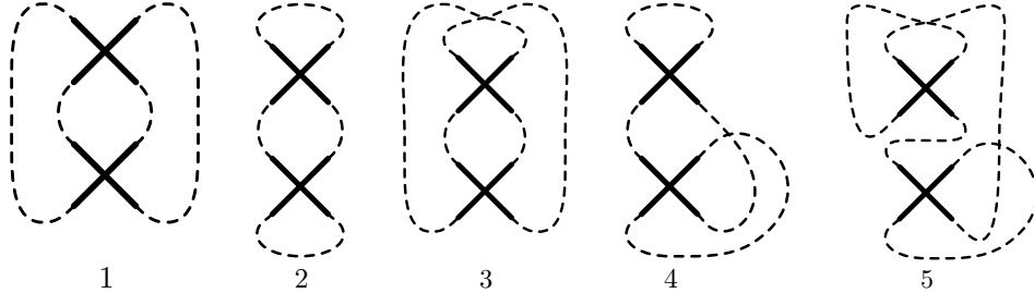
FIGURE 14. Connected shadow diagrams with 2-crossings.
