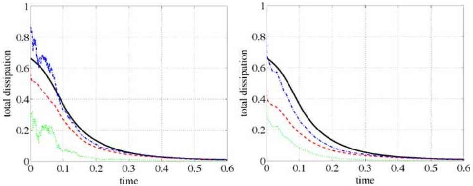
Figure 12. Resolved and SGS dissipation for (left) SCALES with the dynamic model and (right) SCALES with SGS model coefficient C_\epsilon \ell^2 \epsilon^2 = 0.0001 , for Case Re_x=72 with complete adjacent zone. On both plots the DNS viscous dissipation is shown (—) with the viscous dissipation (---), SGS dissipation (-.-.-) and viscous + SGS dissipation (---).
