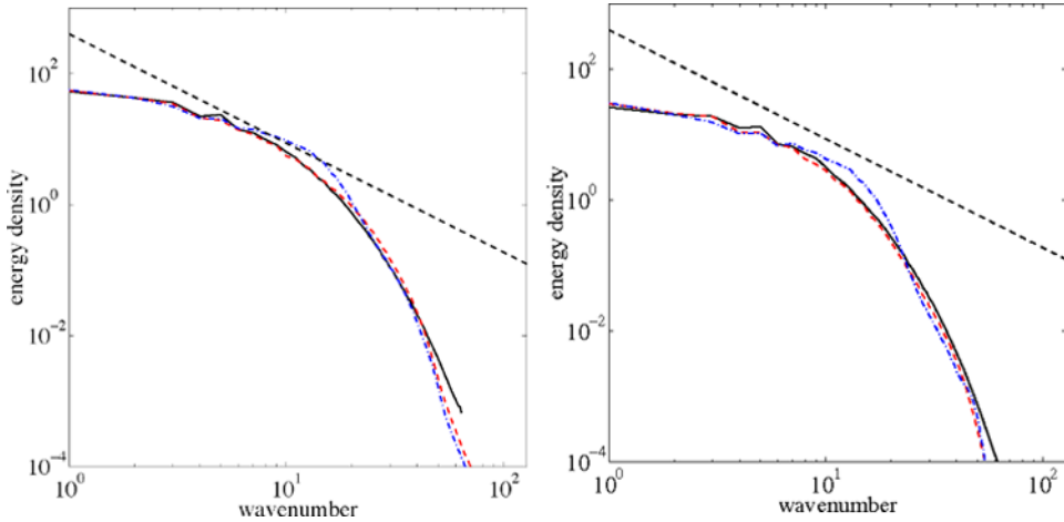
Figure 8. Energy spectra for Case _{Re_\lambda=72} with partial adjacent zone for CVS with no SGS model (— — —), SCALES with no SGS model (— — —) and for comparison DNS (—), at time t = 0.08 (left) and t = 0.16 (right). A k^{-5/3} straight dashed black line is shown to indicate the inertial range.
