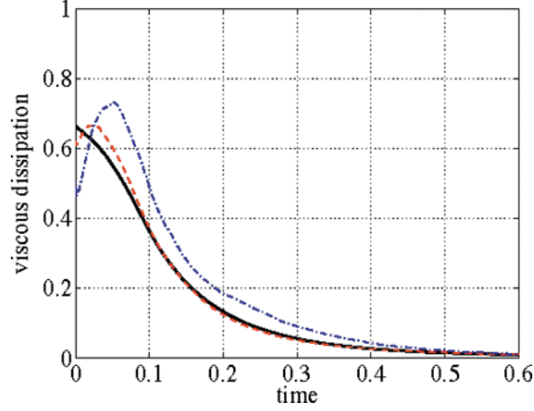
Figure 7. Total resolved viscous dissipation ( -\nu S_{ij} S_{ij} ) for Case _{Re_\lambda=72} with partial adjacent zone for CVS with no SGS model (— — —), SCALES with no SGS model (— — —) and for comparison DNS (—).
