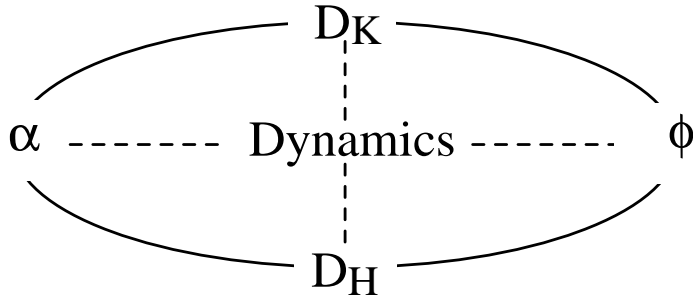
Fig. 2. The relation between quantities important for the analysis of the fine-scale structure of turbulence: the exponent of the Fourier energy spectrum \alpha , Fourier phase spectrum \phi(k) , Kolmogorov capacity D_K , and Hausdorff dimension D_H . The solid lines indicate primarily fixed relationships, while the dotted lines indicate that the relationship is determined by the dynamics of the turbulence.
