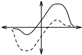
Fig. 1. Typical eddy structure from the test function u(x) = (a + bx) \exp(-x^2) .
