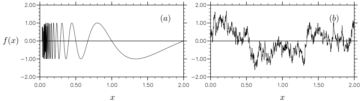
Fig. 3. (a) Original, and (b) scrambled versions of the accumulating function f(x) = \sin(2\pi/x) .
