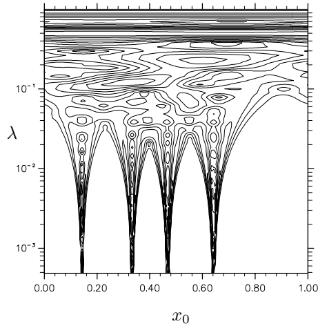
Fig. 6. Branching pattern in the modulus of the Morlet wavelet transform produced by a random superposition of four \sin(2\pi/x) spirals.
