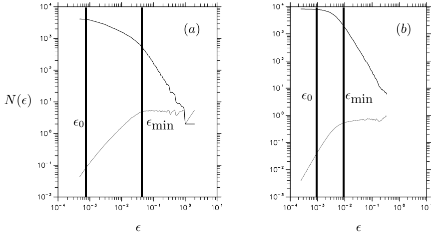
Fig. 4. Calculating the box-counting dimension. (a) Spiral function \sin(2\pi/x) , lower curve is \times \epsilon^{1.5} . (b) Scrambled spiral, lower curve is \times \epsilon^{1.75} . Note the much more gradual transition between \epsilon_{\min} (the lower limit of the power-law section of the curve) and \epsilon_0 (the minimum spacing between points in the signal) for the locally self-similar spiral.
