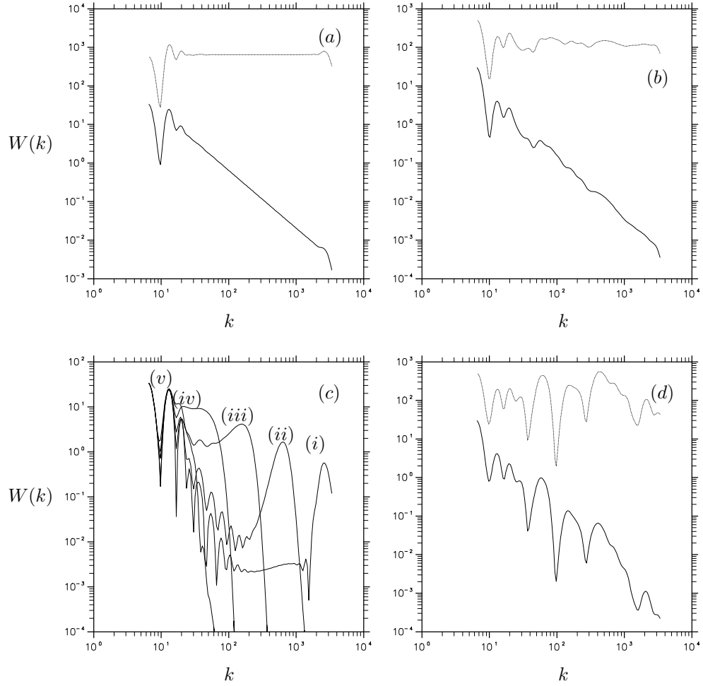
Fig. 5. Distinguishing between locally and globally self-similar signals using the wavelet transform. (a) Wavelet energy spectrum averaged over all locations for the spiral (upper curve is \times k^{1.5} ). (b) Wavelet energy spectrum averaged over all locations for the scrambled spiral (upper curve is \times k^{1.5} ). (c) Local wavelet spectra \times k^{1.5} of the spiral at locations (i) 0.05, (ii) 0.1, (iii) 0.2, (iv) 0.4, (v) 0.8. The flat regions indicate the locations of k^{-1.5} spectrum. (d) Typical local wavelet spectrum of the scrambled spiral at location x = 0.4 (upper curve is \times k^{1.5} ).
