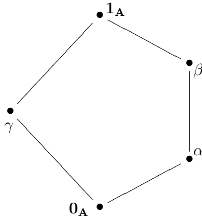
Figure 1: \alpha, \beta , and \gamma
