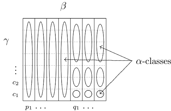
Figure 2: (P \cup Q) \times C
