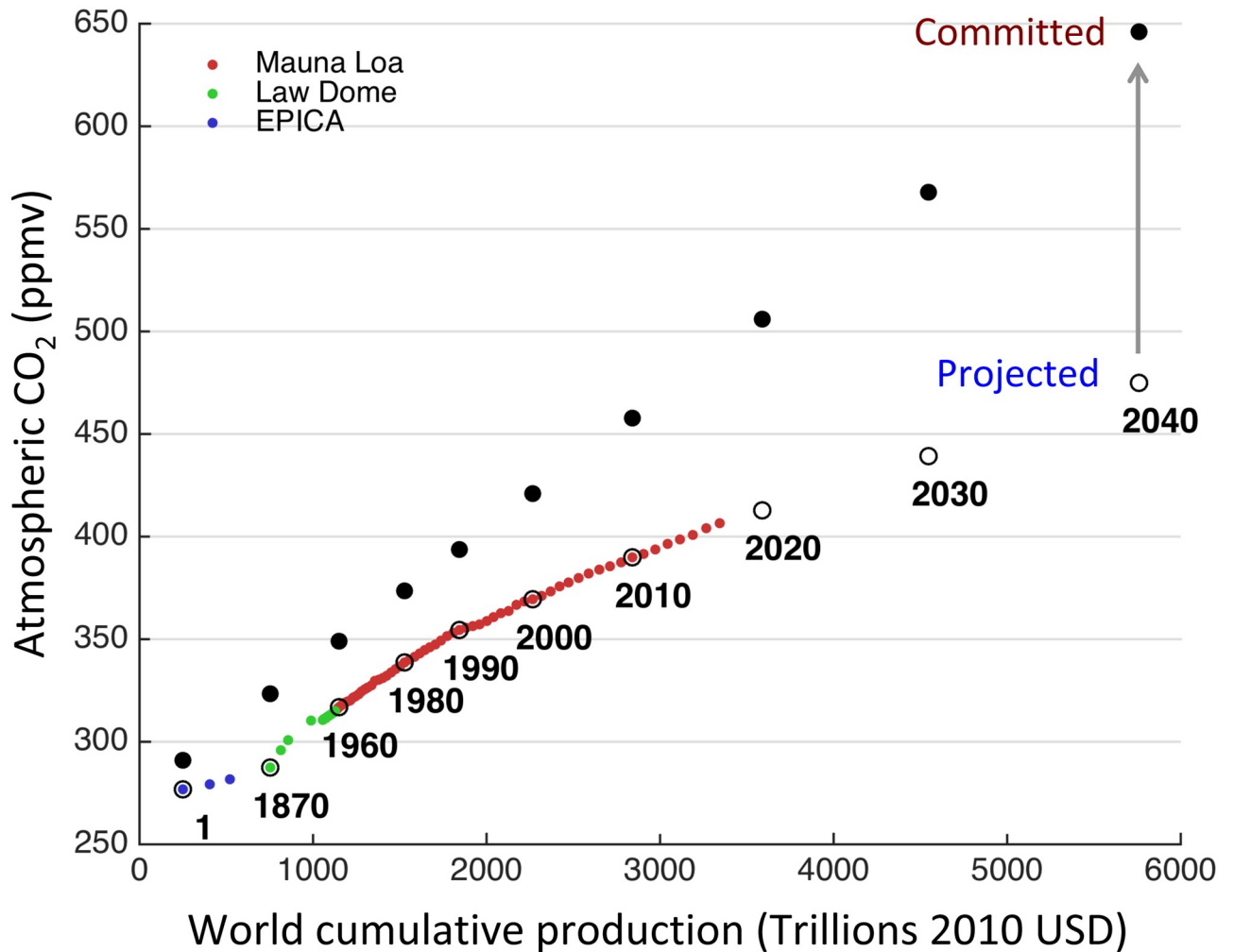
Fig 4. Historical reconstructions of world cumulative production W and atmospheric CO 2 concentrations with projections assuming \eta_c = 0 and \eta_e = \eta_e(2017) = 2.4\%yr^{-1} (circles) and corresponding stabilization concentrations from Eq 39. The halving time between predicted and committed is about 30 years. Concentration data includes flask samples from Mauna Loa [41] and Antarctic ice core data [42, 43].
