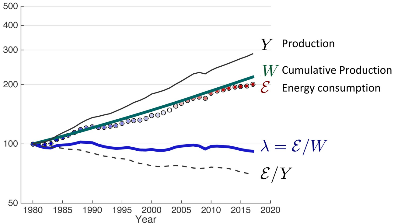
Fig 3. Relative evolution since 1980 of the world real GDP Y , economic potential W = \int_0^t Y(t')dt' (Eq 19), primary energy consumption \mathcal{E} , \lambda = \mathcal{E}/W (Eq 18) and the energy intensity of production i =: \mathcal{E}/Y = 1/\lambda .
